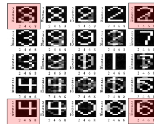
Train a 5x5 Kohonen feature map. Then take the four corner units as our RBF centers.
