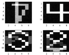
Four RBF centers trained by k-means clustering.
