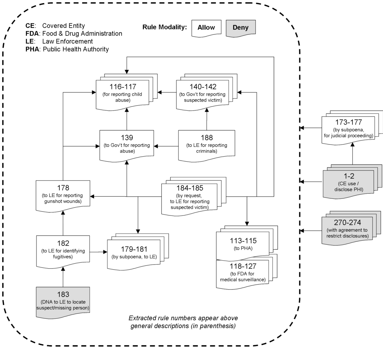
Fig. 6. Example network of priorities between rules.
